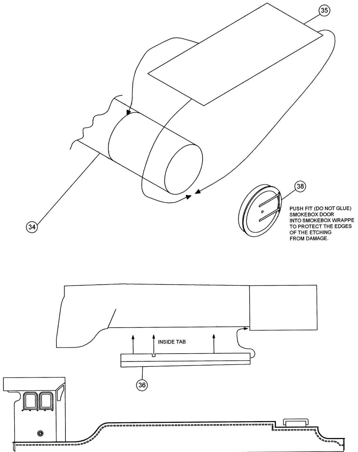
FIG. 3. BOILER PREPARATION.
