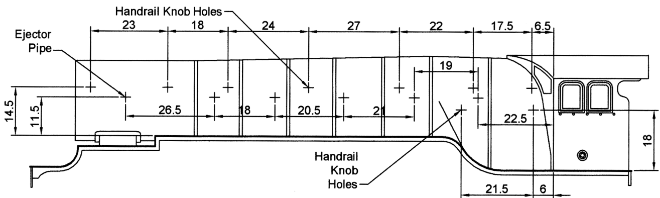
Diagram 118 Boiler
